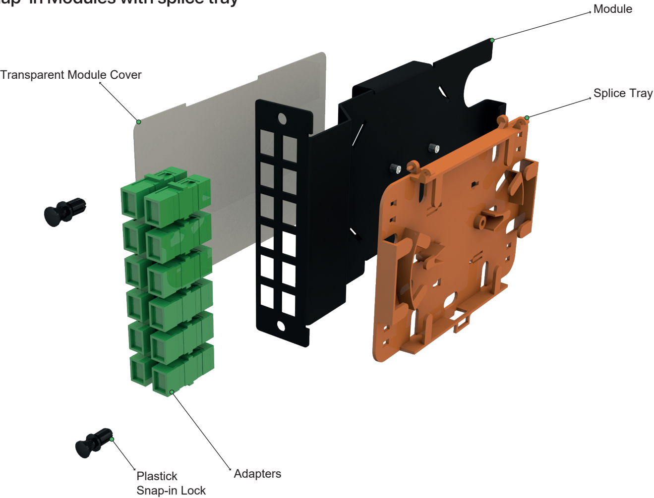
Snap-in Modules with splice tray
